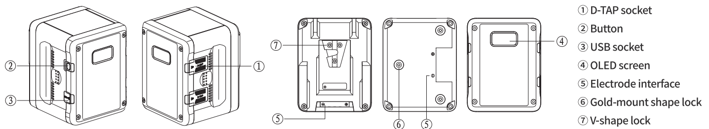
Fig 1: PB-S220S/A
